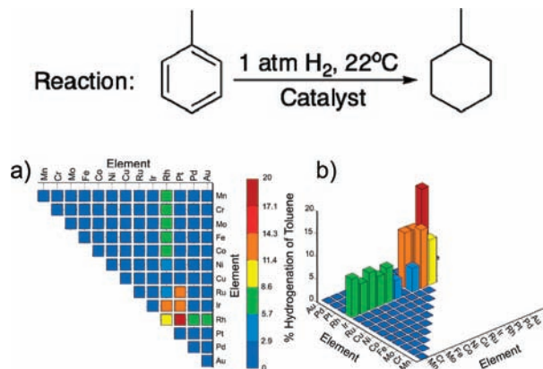
Figure 1. 3D bar graphs (a, top down view) and (b, side view) of screening results. The x - and y - axes represent the different transition metals used, with the z -axis showing the percent hydrogenation after 4 h.
